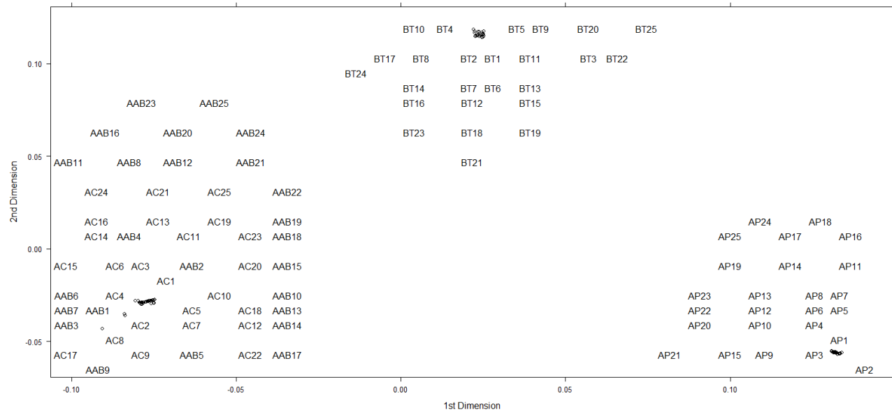
Figure 12: Multidimensional scaling plot of cytb , CoxI , and D-loop region for all four native wild deer species.
