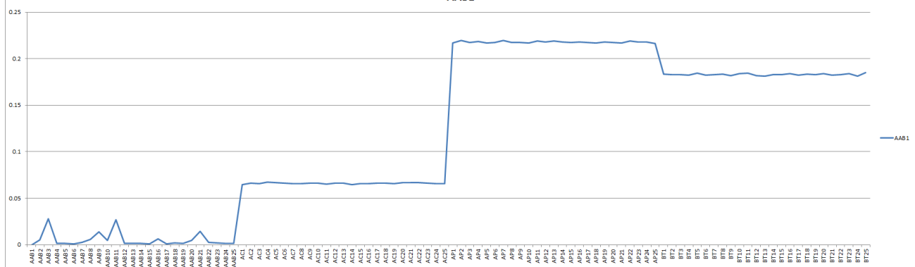
Figure 13: Cyb , CoxI , and D-loop region-based variation plot of the studied four wild deer species.
