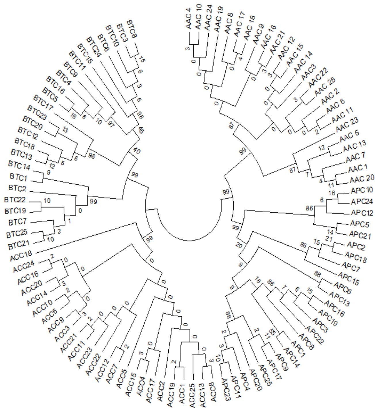
Figure 5: Phylogenetic tree (circular) of the Cox1 gene of the studied species ( Boselaphus tragocamelus , Antilope cervicapra , Axis axis , and Axis porcinus ).
