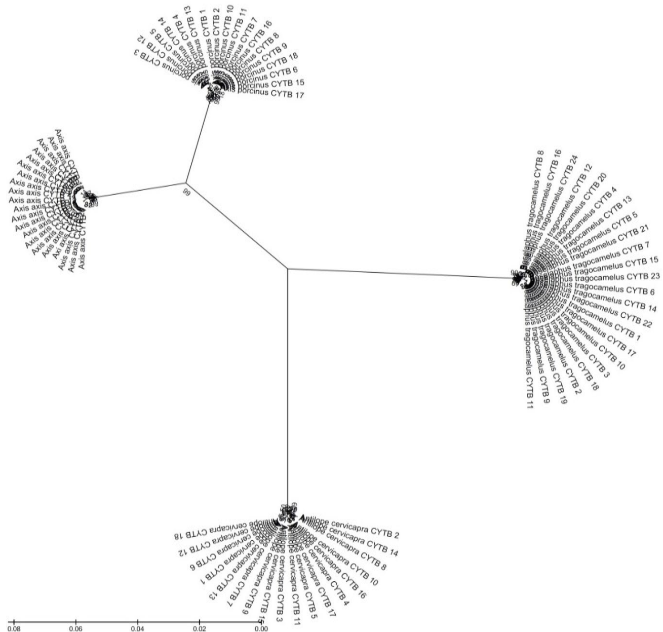
Figure 2: Phylogenetic tree (radiation) of the cytb gene of studied four wild deer species ( Boselaphus tragocamelus , Antelope cervicapra , Axis axis , and Axis porcinus ).
