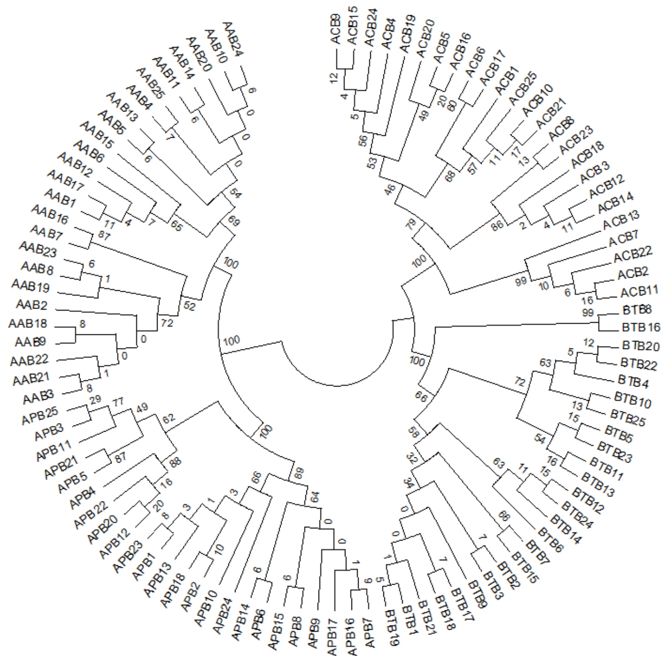
Figure 3: Phylogenetic tree (circular) of the cytb gene (collectively) of the studied four wild deer species ( Boselaphus tragocamelus , Antelope cervicapra , Axis axis , and Axis porcinus ).
