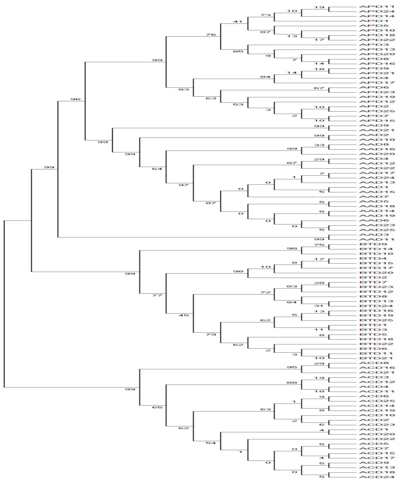
Figure 6: Phylogenetic tree (rectangular) of the D-loop region of the studied species ( Boselaphus tragocamelus , Antelope cervicapra , Axis axis , and Axis porcinus ).
