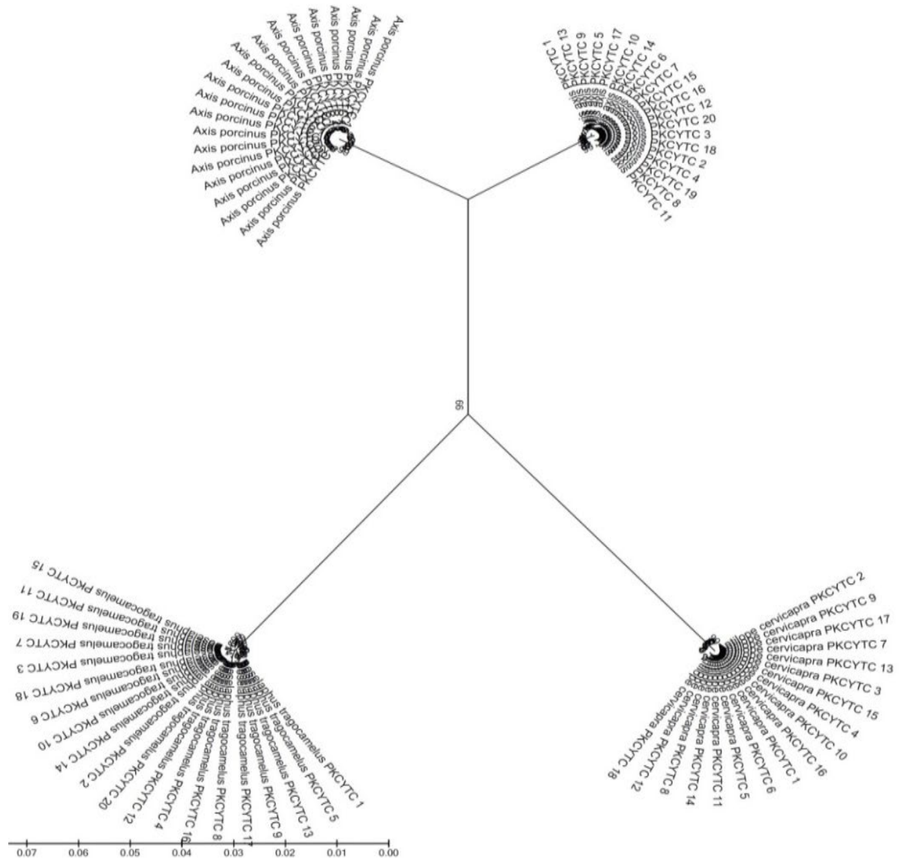
Figure 4: Phylogenetic tree (radiation) of the Cox1 gene (collectively) of the studied species ( Boselaphus tragocamelus , Antelope cervicapra , Axis axis , and Axis porcinus ).
