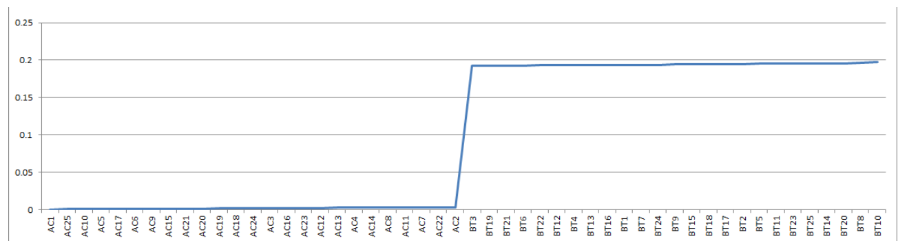
Figure 9: Cytb , Cox1 , and D-loop region-based genetic variation plot of Bovidae ( Boselaphus tragocamelus and Antelope cervicapra ).
