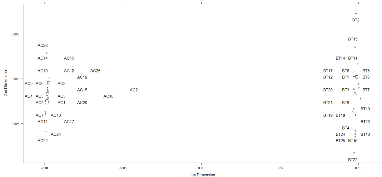
Figure 8: Multidimensional scaling plot of cytb , Cox1 , and D-loop region for Bovidae ( Boselaphus tragocamelus and Antelope cervicapra ).
