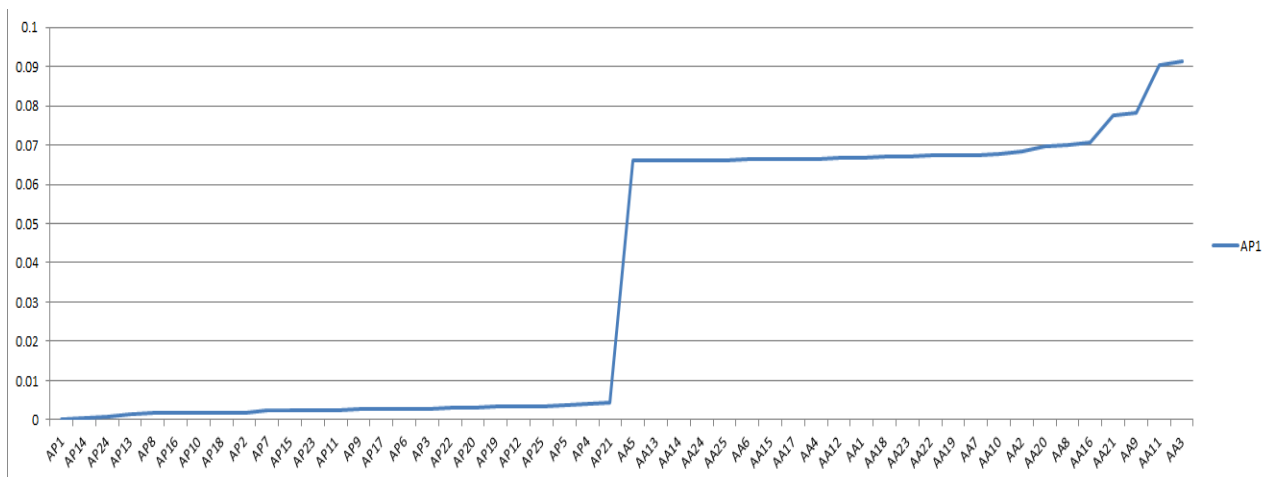
Figure 11: Cytb , Cox1 , and D-loop region-based genetic variation plot of Cervidae ( Axis axis and Axis porcinus )
