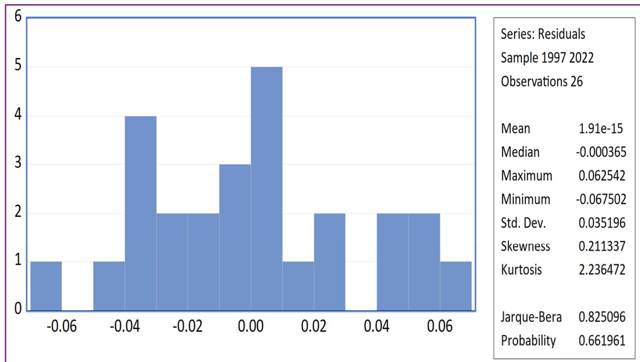
Figure 1: Jarque-Bera expected distribution test results.
