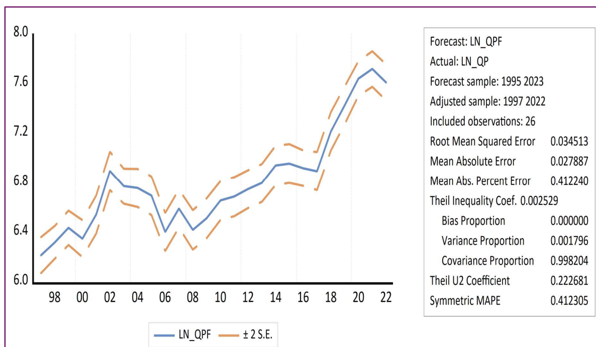
Figure 4: Results of the model's predictive power Test.
