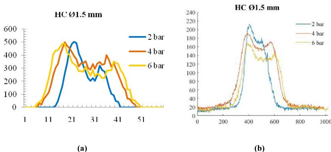
Figure 3. Spray patterns (a) CMEIAS Image Tool Ver. 1.28, (b) MATLAB R2009a
